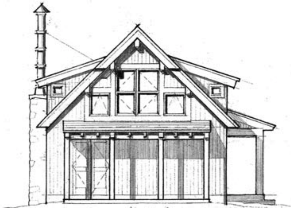
LEFT ELEVATION
